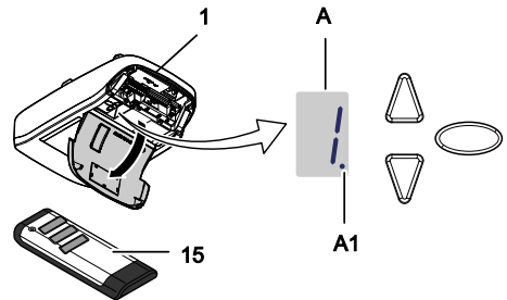
Fig. 4: Control elements
