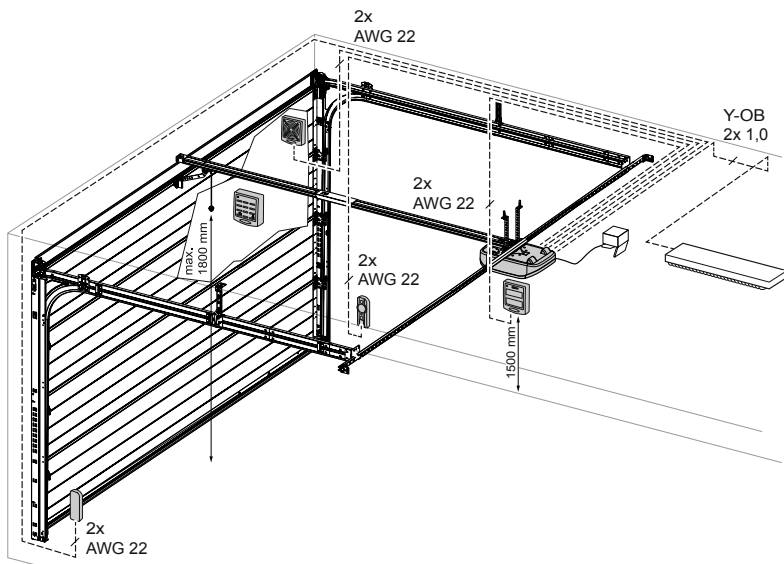
Fig. 3: Example installation of accessories
